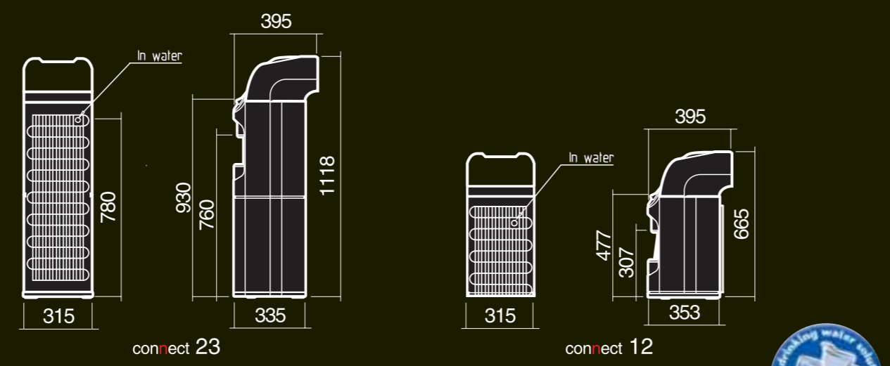
connect 23 connect 12
